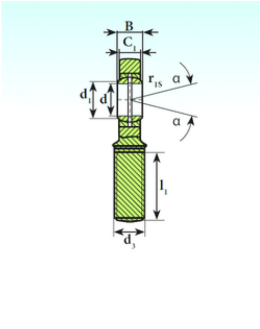
SA 45 ES 2RS Bearing 2D drawings and 3D CAD models
