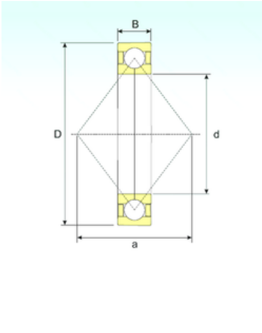
QJ 1264 Bearing 2D drawings and 3D CAD models
