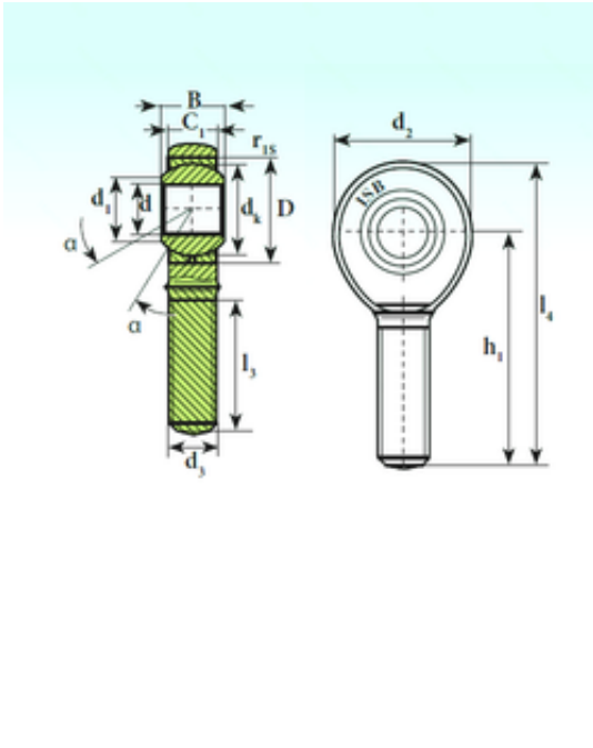
TSM 12.1 C Bearing 2D drawings and 3D CAD models
