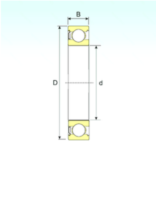
6002-Z Bearing 2D drawings and 3D CAD models
