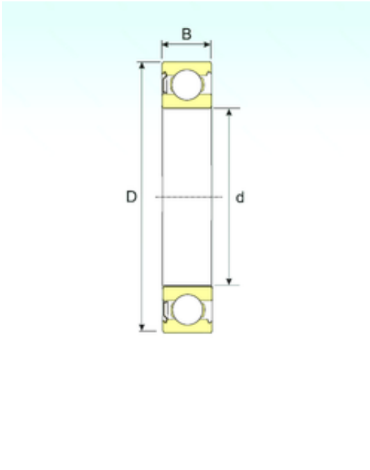
6303-Z Bearing 2D drawings and 3D CAD models
